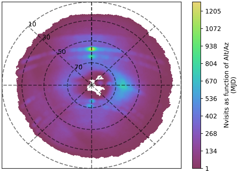
no_high_blob_v3.3_10yrs g band: Nvisits as function of Alt/Az
