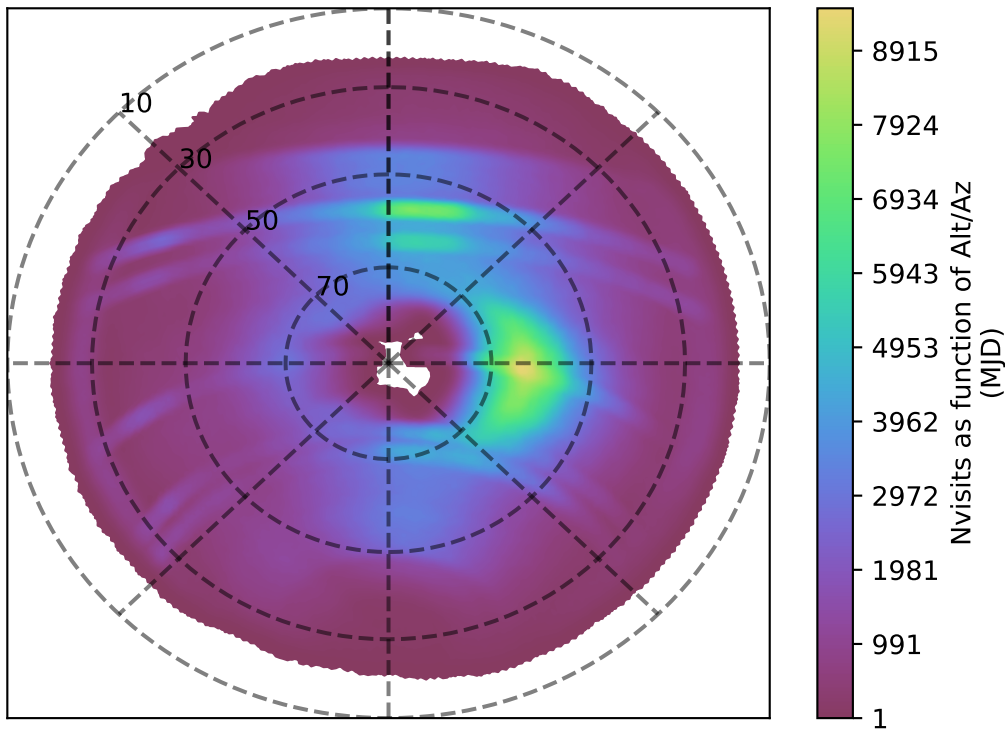
no_high_blob_v3.3_10yrs all bands: Nvisits as function of Alt/Az
