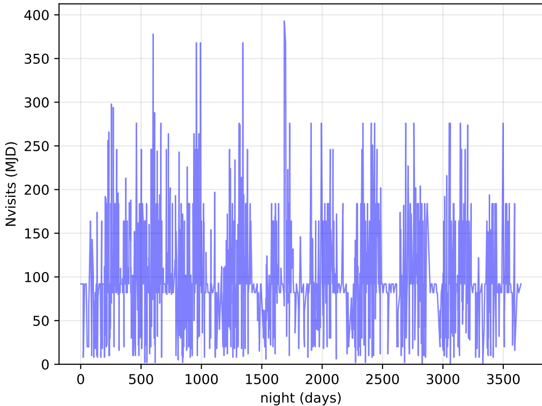
no_high_blob_v3.3_10yrs DDF: Nvisits
