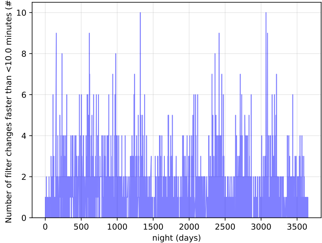
no_high_blob_v3.3_10yrs Per Night: Number of filter changes faster than <10.0 minutes
