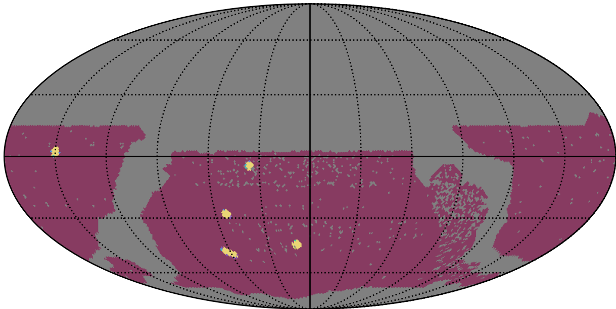
no_high_blob_v3.3_10yrs WFD: NumberOfQuickRevisits
