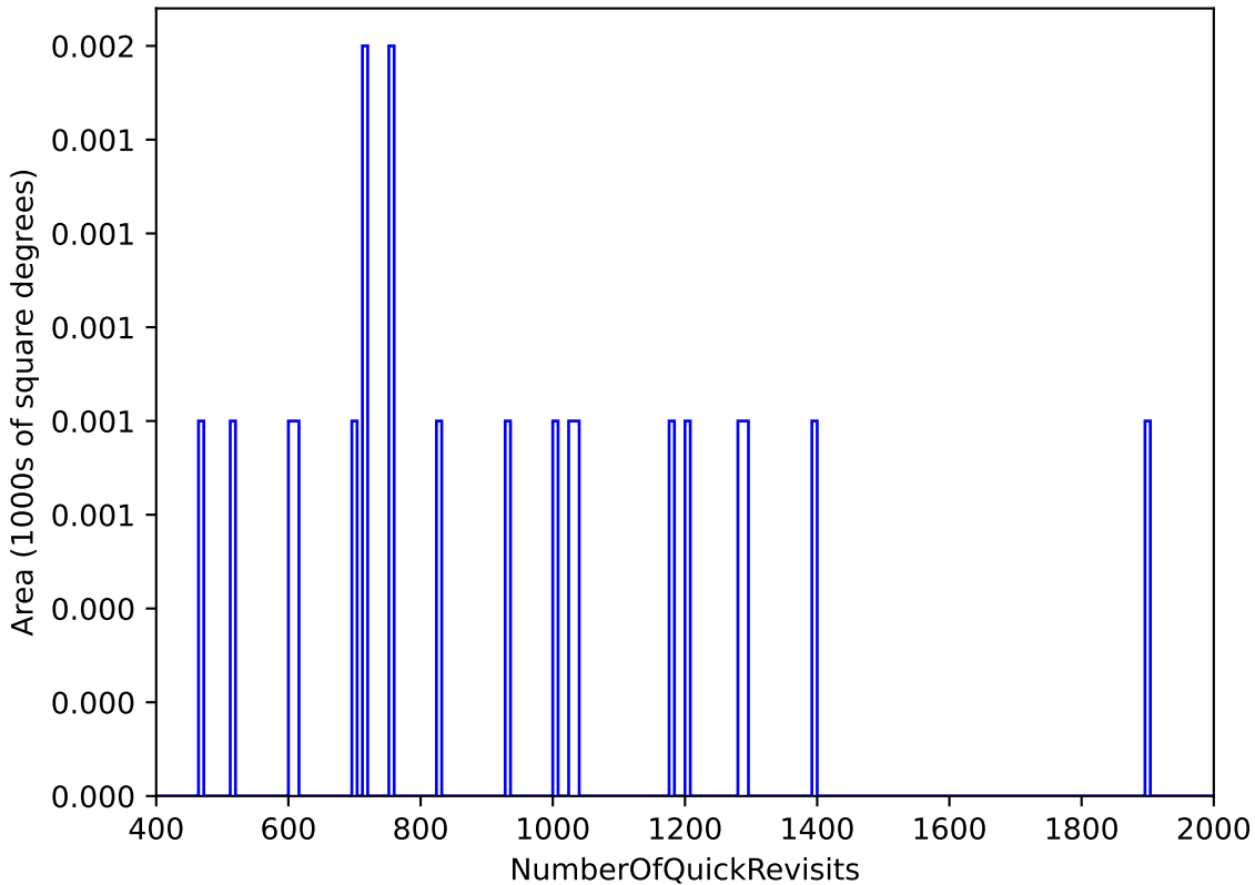
no_high_blob_v3.3_10yrs WFD: NumberOfQuickRevisits
