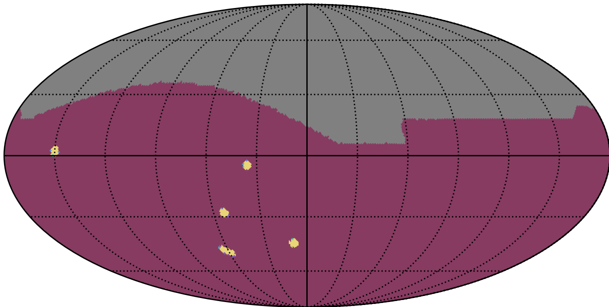
no_high_blob_v3.3_10yrs All sky: NumberOfQuickRevisits
