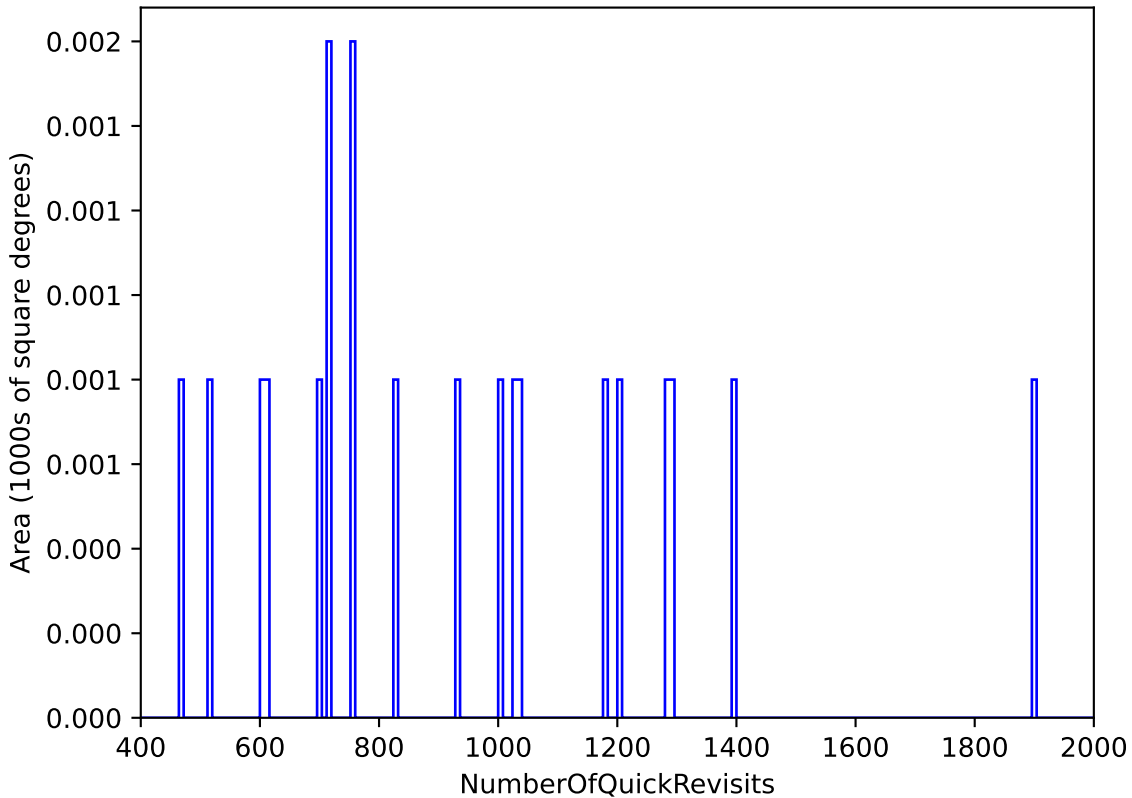
no_high_blob_v3.3_10yrs All sky: NumberOfQuickRevisits
