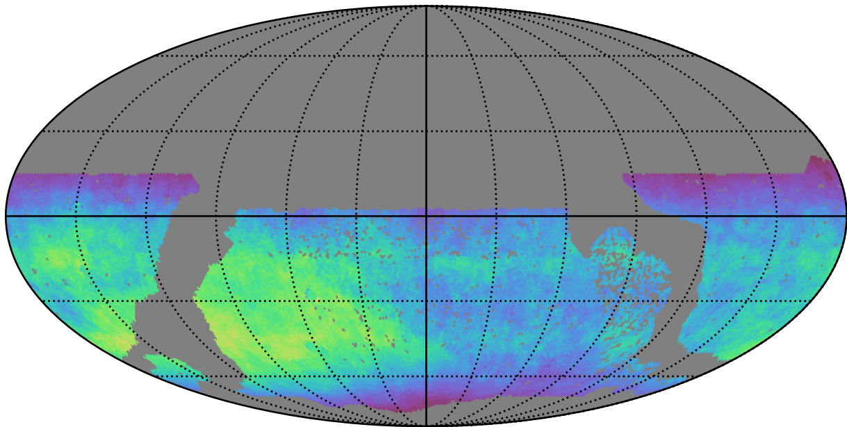
no_high_blob_v3.3_10yrs WFD z band: Normalized Teff
