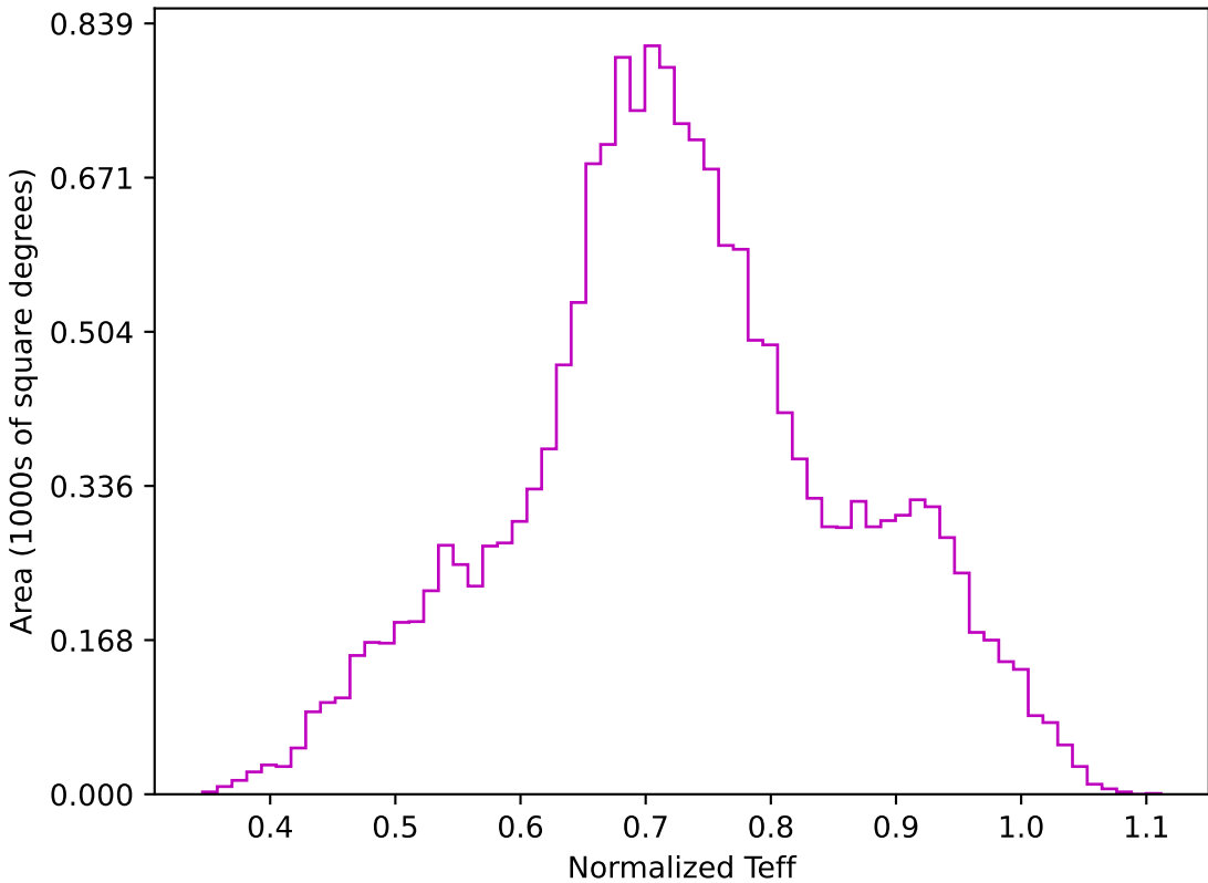
no_high_blob_v3.3_10yrs WFD z band: Normalized Teff
