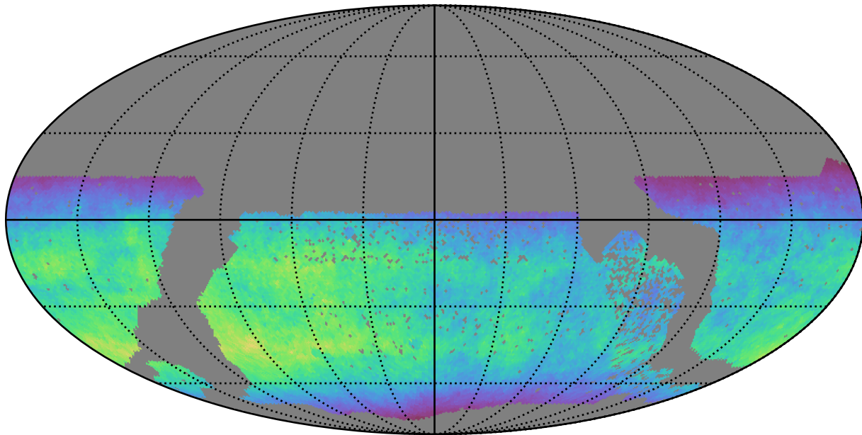
no_high_blob_v3.3_10yrs WFD y band: Normalized Teff
