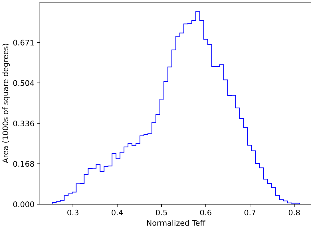
no_high_blob_v3.3_10yrs WFD y band: Normalized Teff
