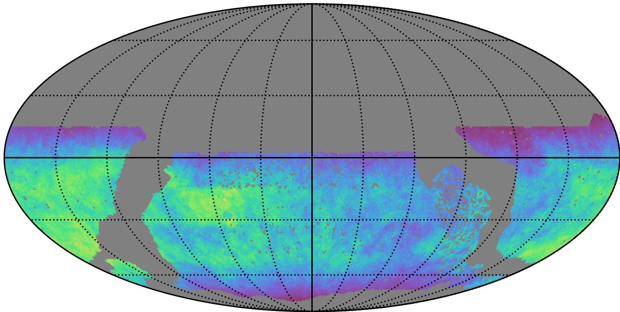
no_high_blob_v3.3_10yrs WFD u band: Normalized Teff
