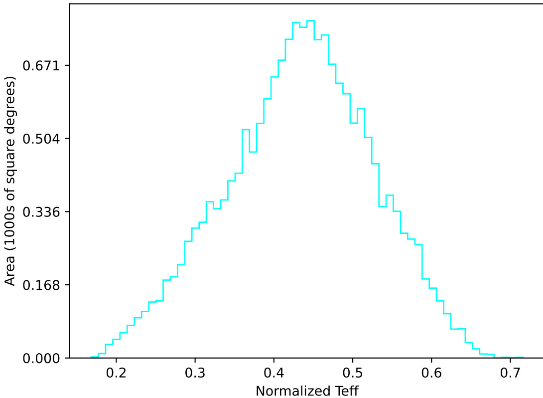
no_high_blob_v3.3_10yrs WFD u band: Normalized Teff
