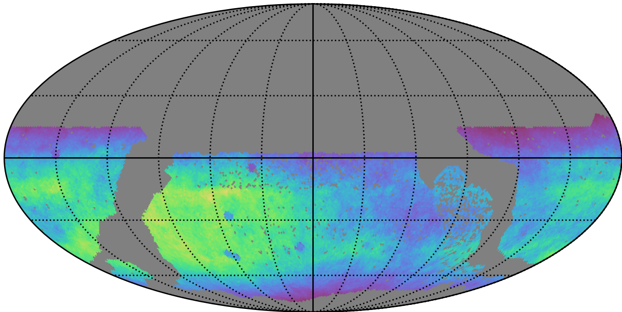
no_high_blob_v3.3_10yrs WFD r band: Normalized Teff
