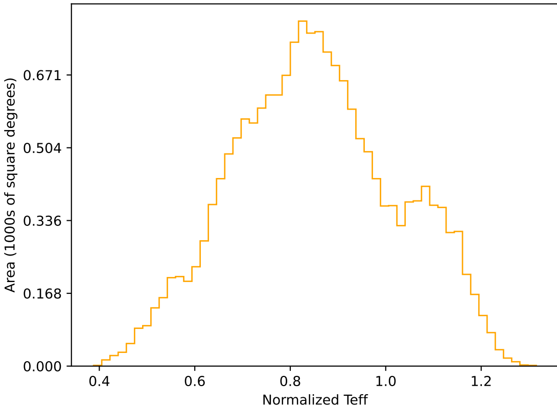
no_high_blob_v3.3_10yrs WFD r band: Normalized Teff
