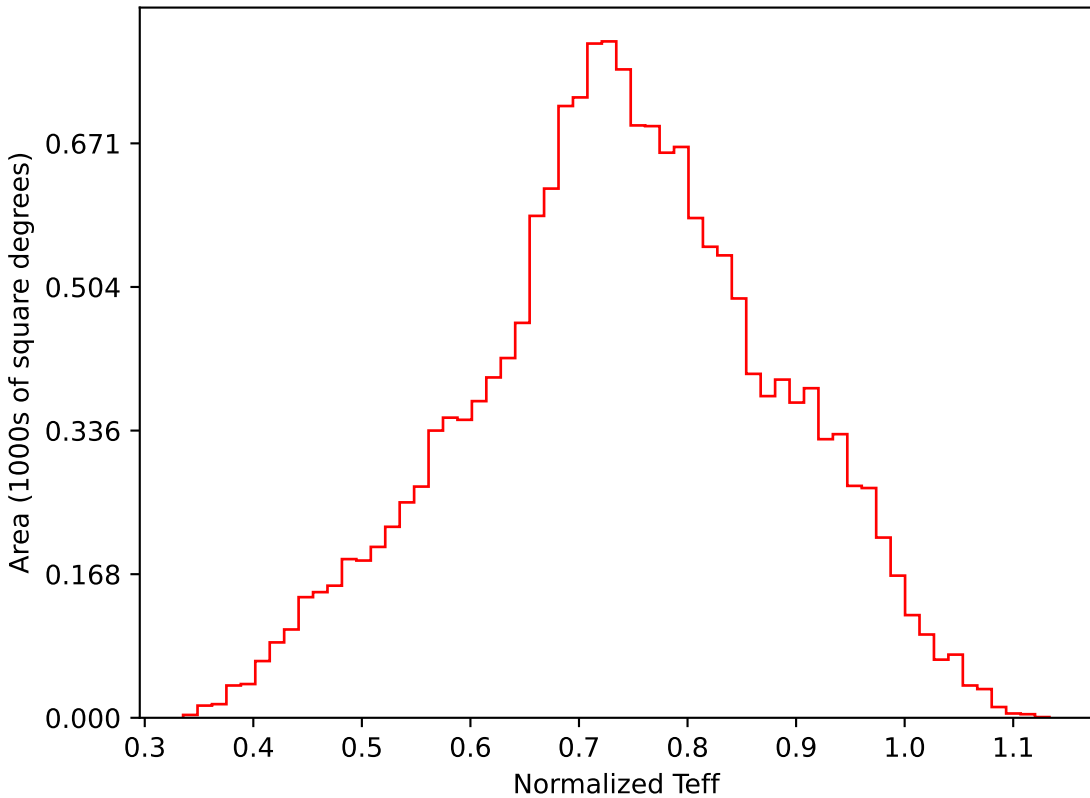
no_high_blob_v3.3_10yrs WFD i band: Normalized Teff
