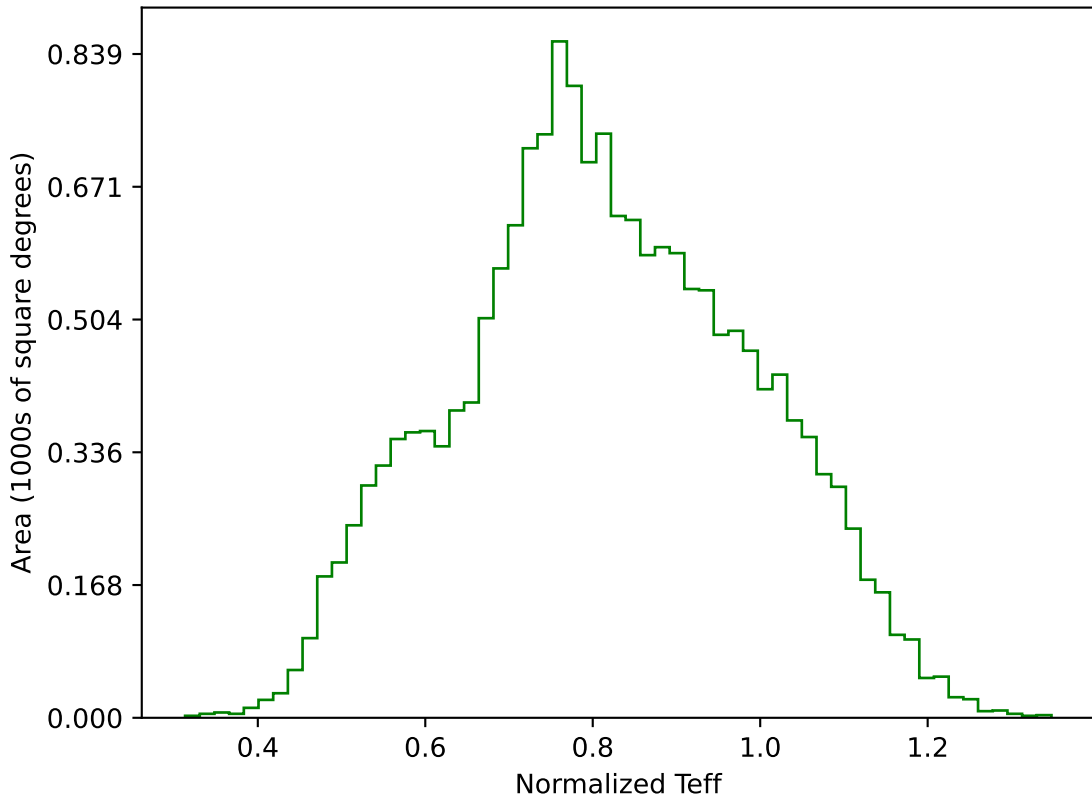
no_high_blob_v3.3_10yrs WFD g band: Normalized Teff
