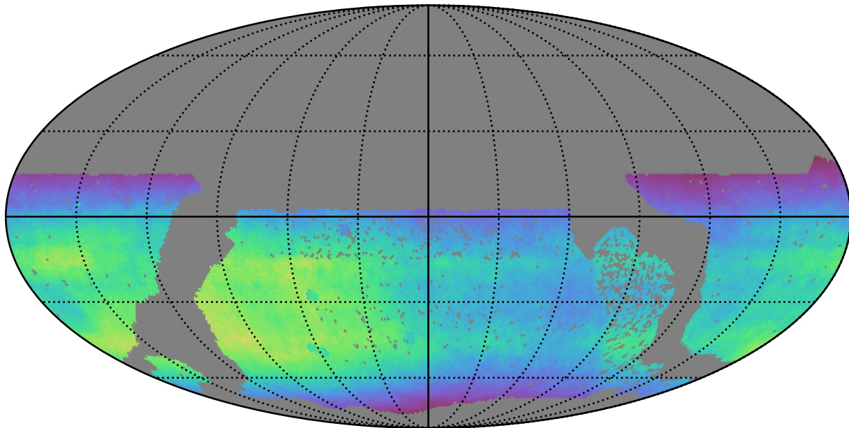
no_high_blob_v3.3_10yrs WFD all bands: Normalized Teff
