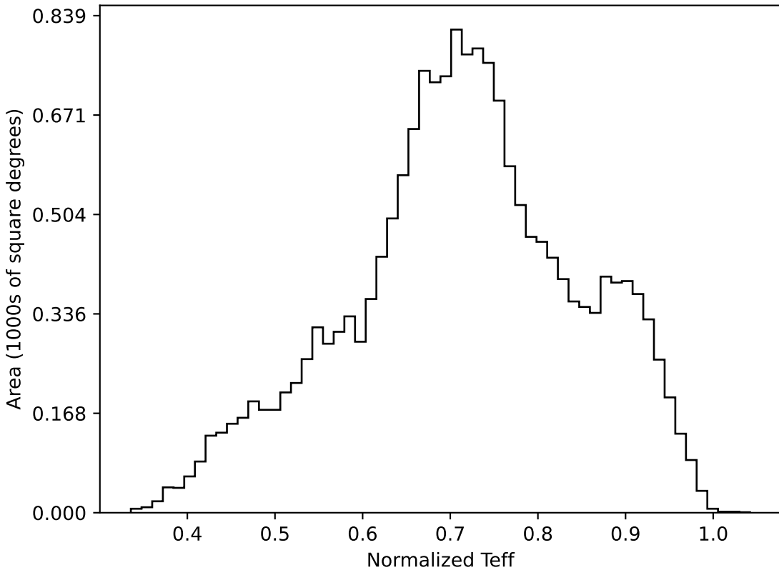
no_high_blob_v3.3_10yrs WFD all bands: Normalized Teff
