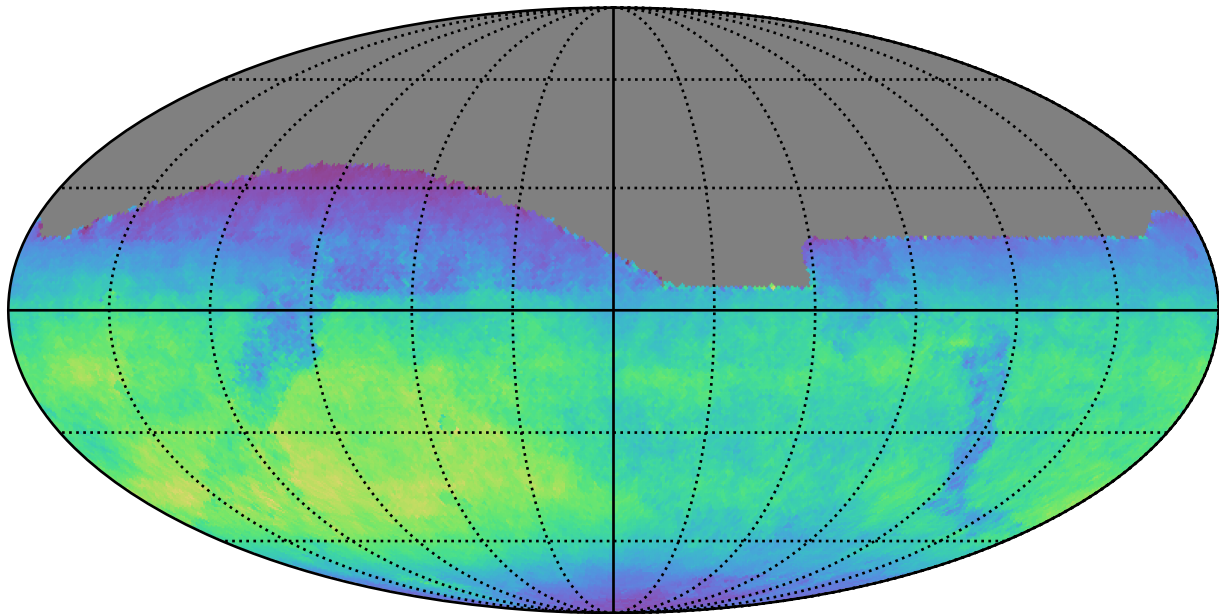
no_high_blob_v3.3_10yrs All sky z band: Normalized Teff
