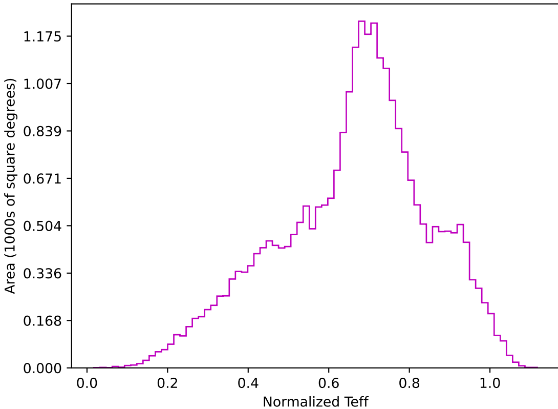
no_high_blob_v3.3_10yrs All sky z band: Normalized Teff
