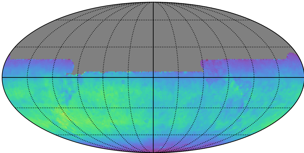
no_high_blob_v3.3_10yrs All sky y band: Normalized Teff
