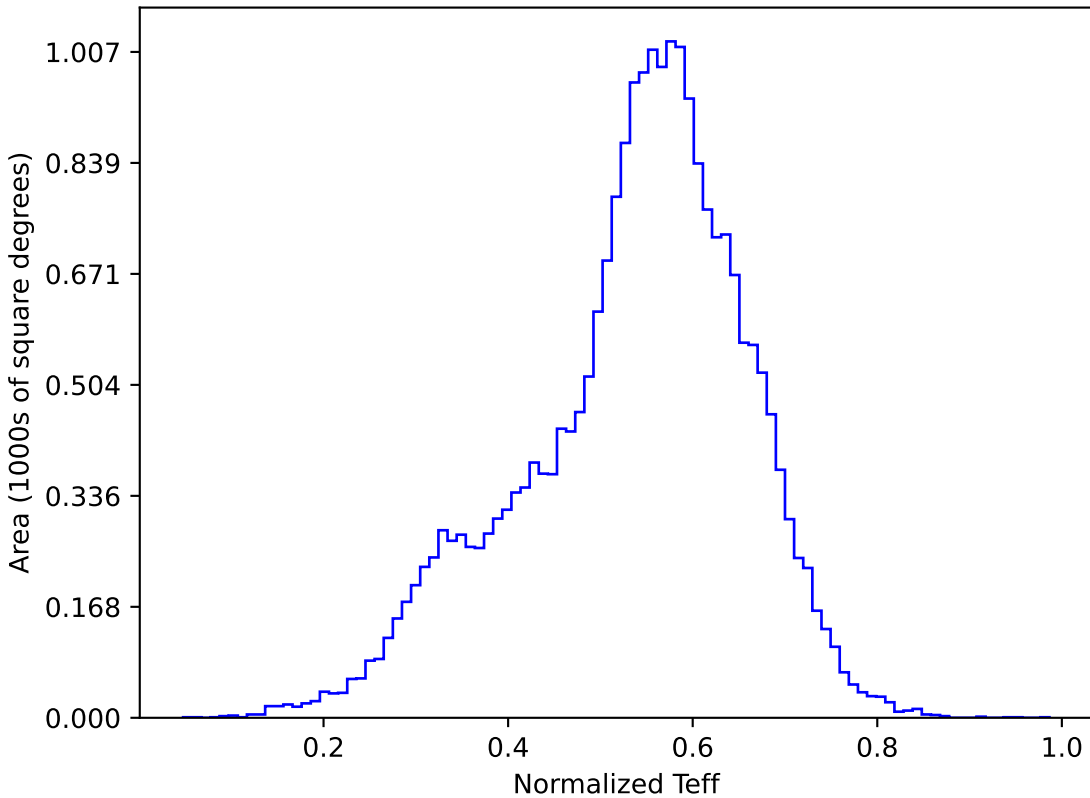
no_high_blob_v3.3_10yrs All sky y band: Normalized Teff
