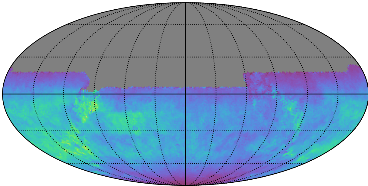
no_high_blob_v3.3_10yrs All sky u band: Normalized Teff
