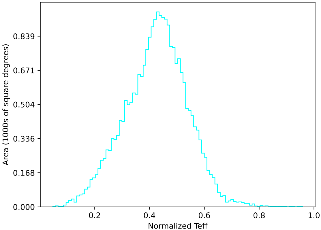
no_high_blob_v3.3_10yrs All sky u band: Normalized Teff
