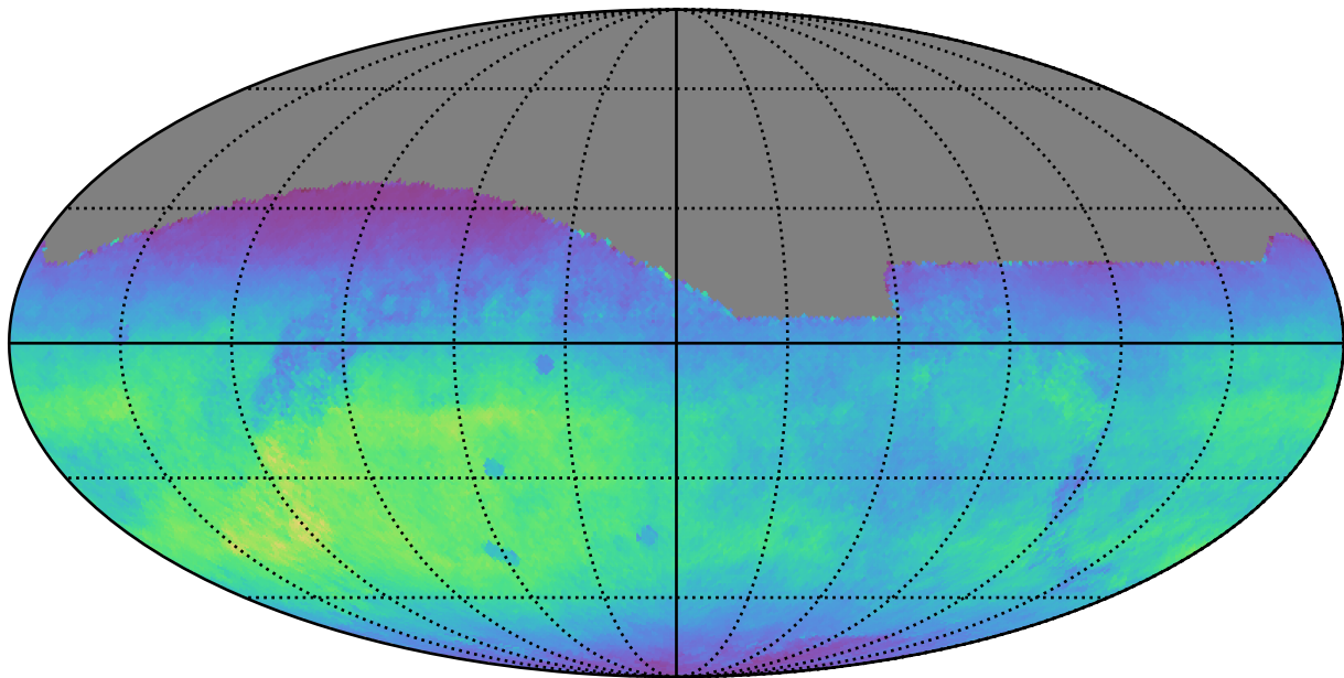
no_high_blob_v3.3_10yrs All sky r band: Normalized Teff
