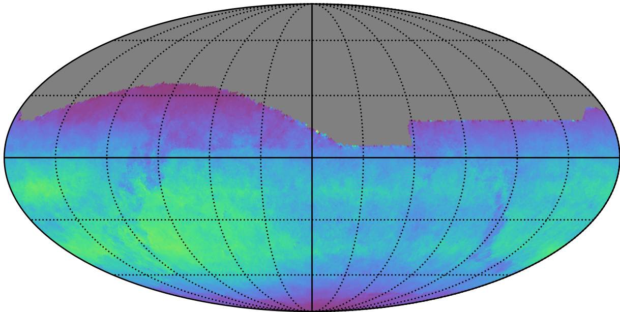
no_high_blob_v3.3_10yrs All sky i band: Normalized Teff
