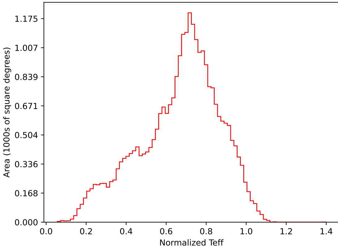
no_high_blob_v3.3_10yrs All sky i band: Normalized Teff
