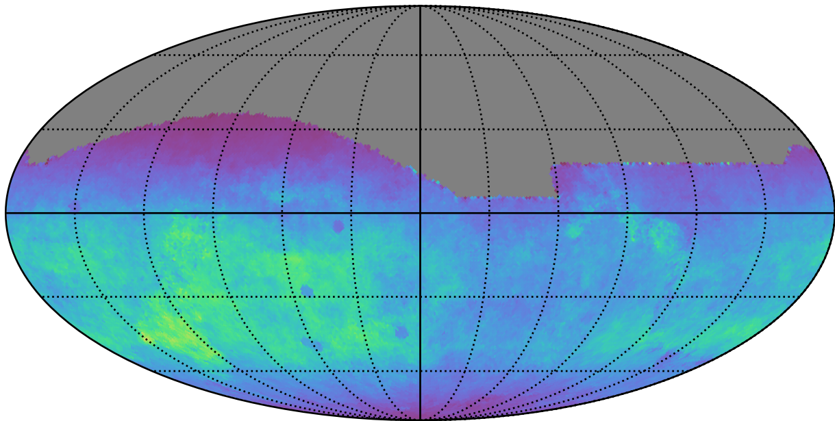
no_high_blob_v3.3_10yrs All sky g band: Normalized Teff
