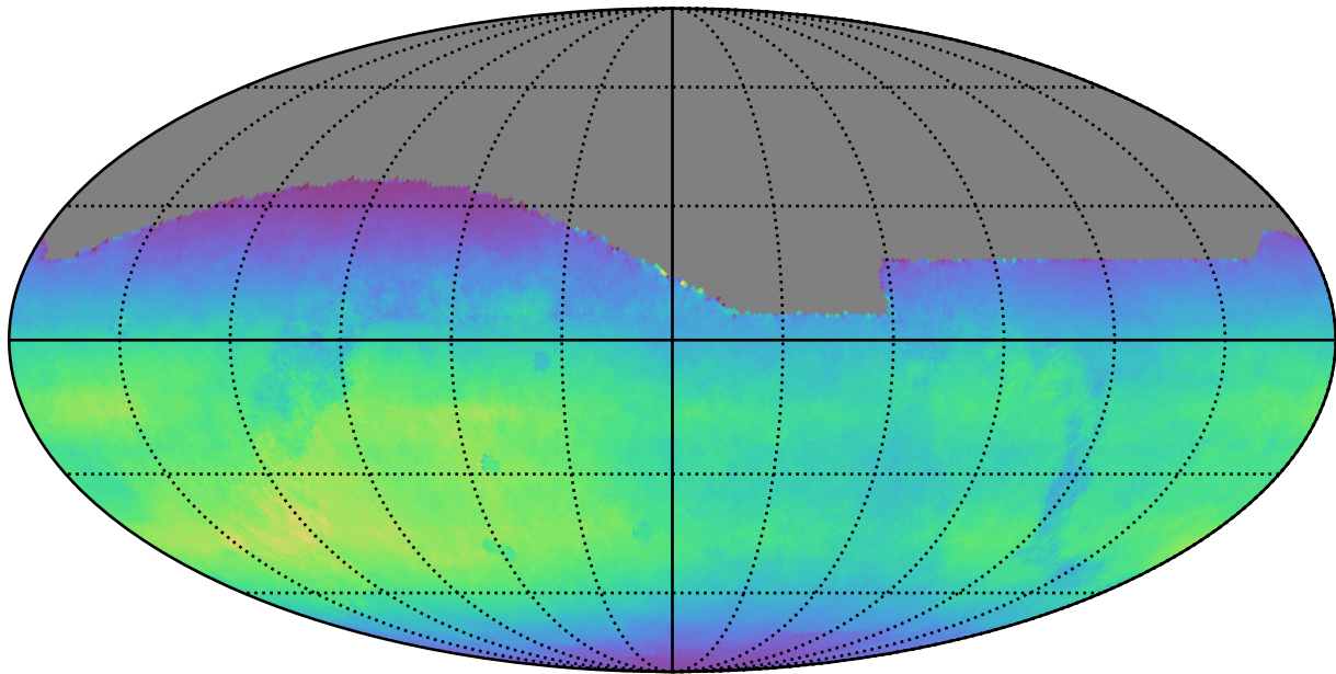
no_high_blob_v3.3_10yrs All sky all bands: Normalized Teff
