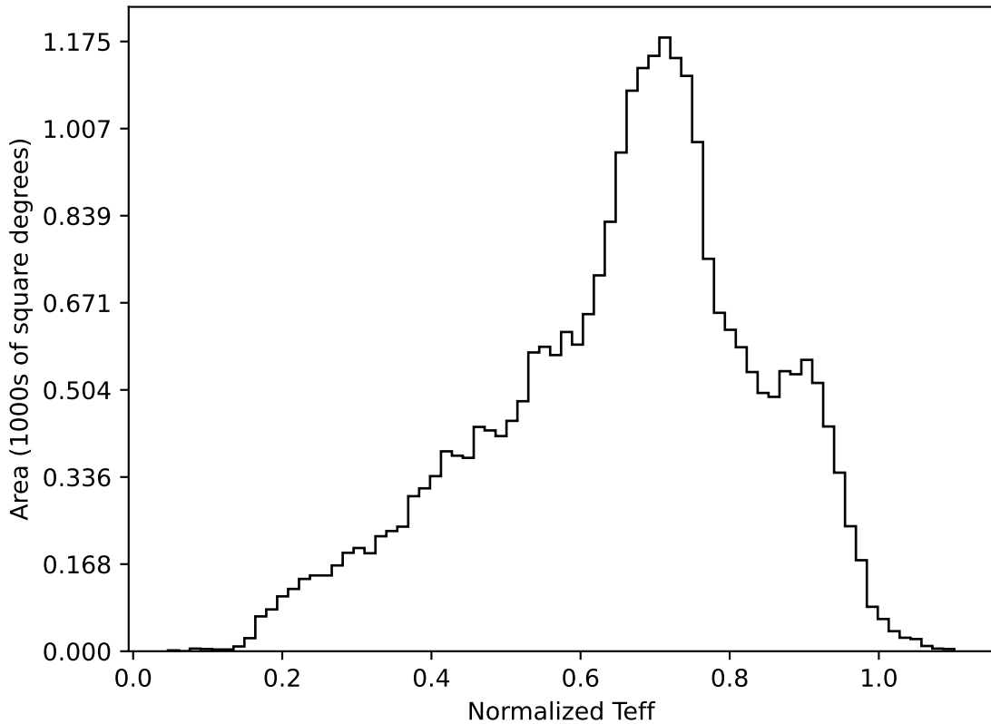
no_high_blob_v3.3_10yrs All sky all bands: Normalized Teff
