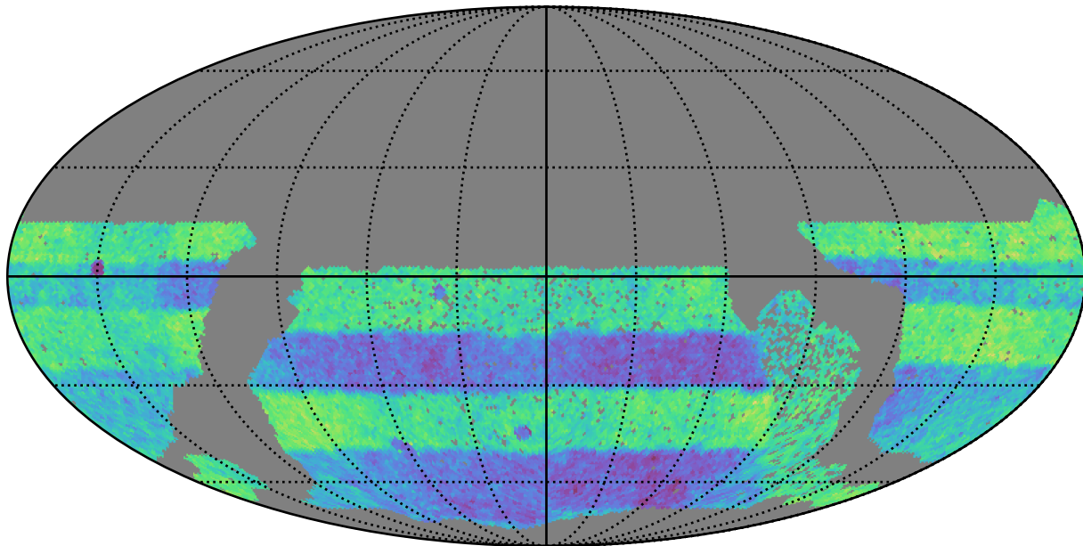
no_high_blob_v3.3_10yrs WFD: Normalized Proper Motion Uncert @ 20.5
