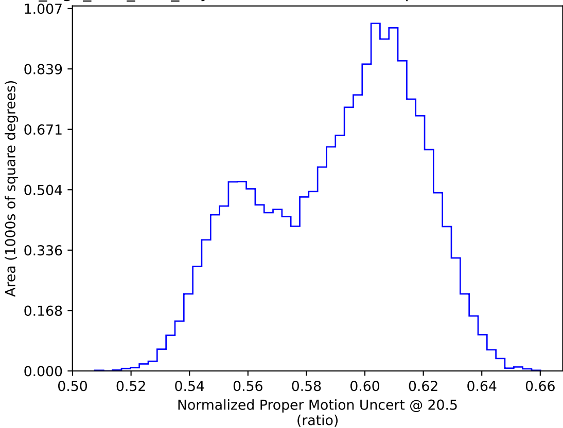
no_high_blob_v3.3_10yrs WFD: Normalized Proper Motion Uncert @ 20.5
