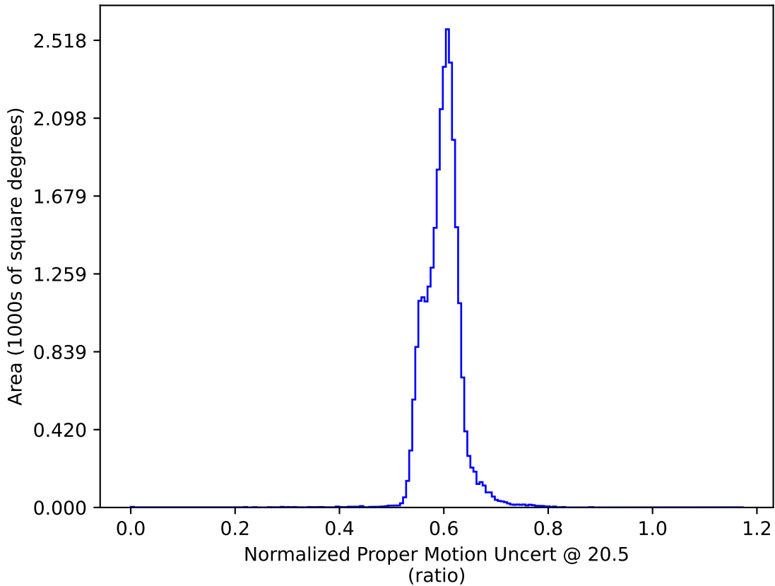
no_high_blob_v3.3_10yrs All sky: Normalized Proper Motion Uncert @ 20.5
