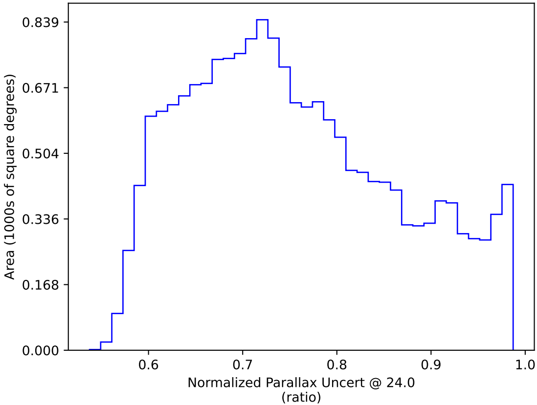
no_high_blob_v3.3_10yrs WFD: Normalized Parallax Uncert @ 24.0
