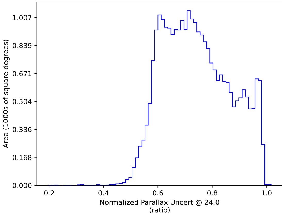
no_high_blob_v3.3_10yrs All sky: Normalized Parallax Uncert @ 24.0
