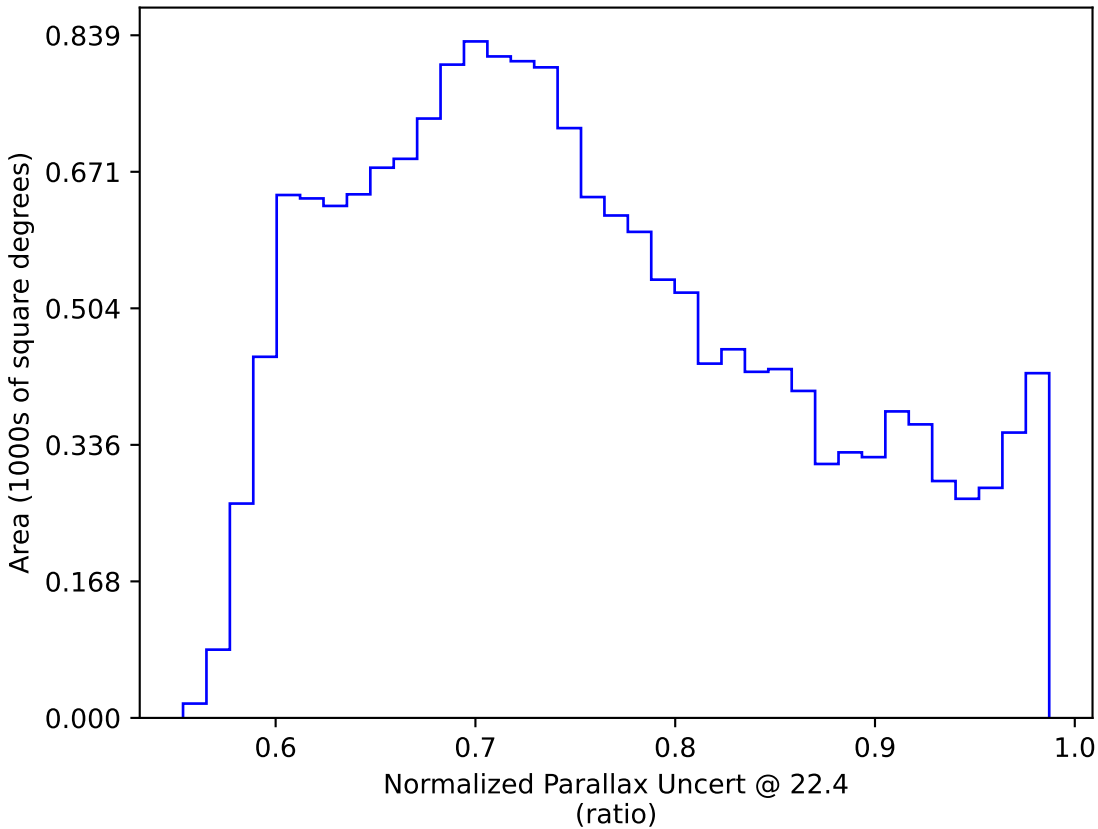
no_high_blob_v3.3_10yrs WFD: Normalized Parallax Uncert @ 22.4
