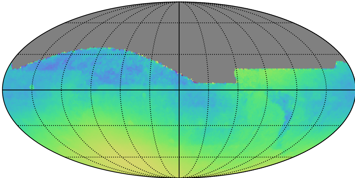
no_high_blob_v3.3_10yrs All sky: Normalized Parallax Uncert @ 22.4
