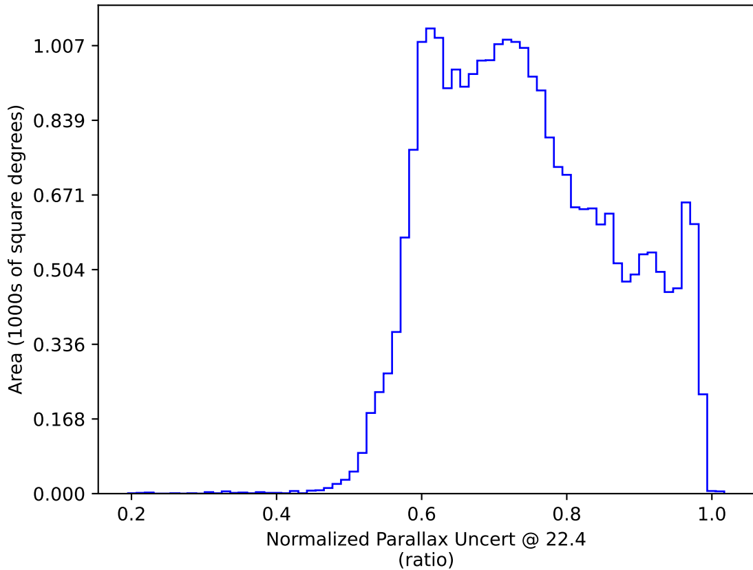
no_high_blob_v3.3_10yrs All sky: Normalized Parallax Uncert @ 22.4
