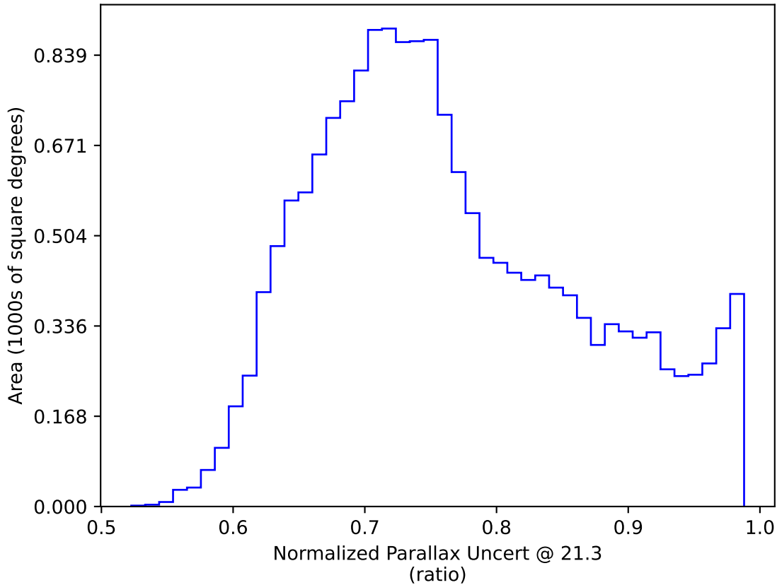
no_high_blob_v3.3_10yrs WFD y band only: Normalized Parallax Uncert @ 21.3
