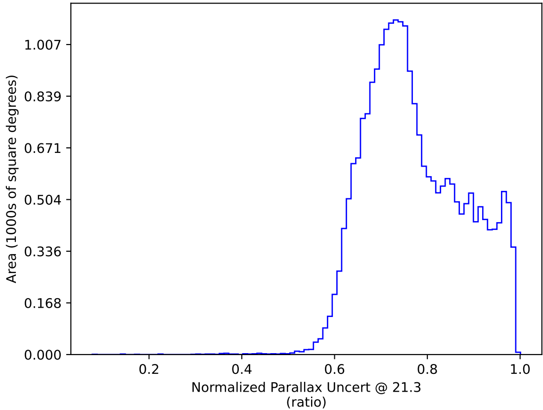
no_high_blob_v3.3_10yrs All sky y band only: Normalized Parallax Uncert @ 21.3
