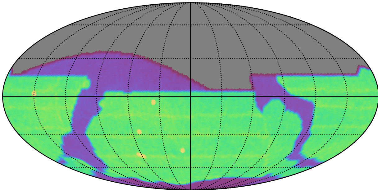
no_high_blob_v3.3_10yrs All sky all bands: N Unique Nights
