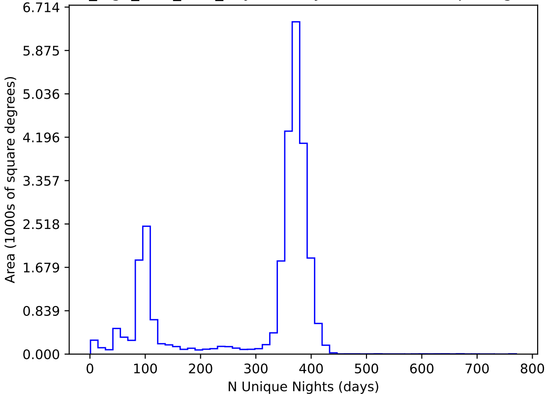
no_high_blob_v3.3_10yrs All sky all bands: N Unique Nights
