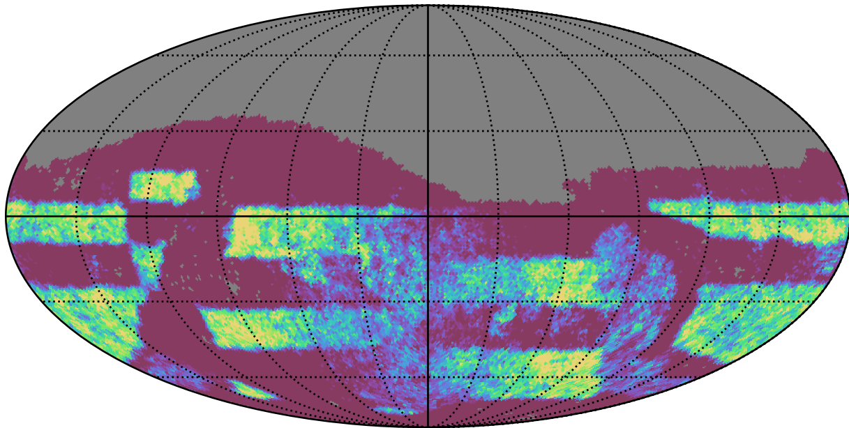
no_high_blob_v3.3_10yrs Yr 3-4 z band: NVisits
