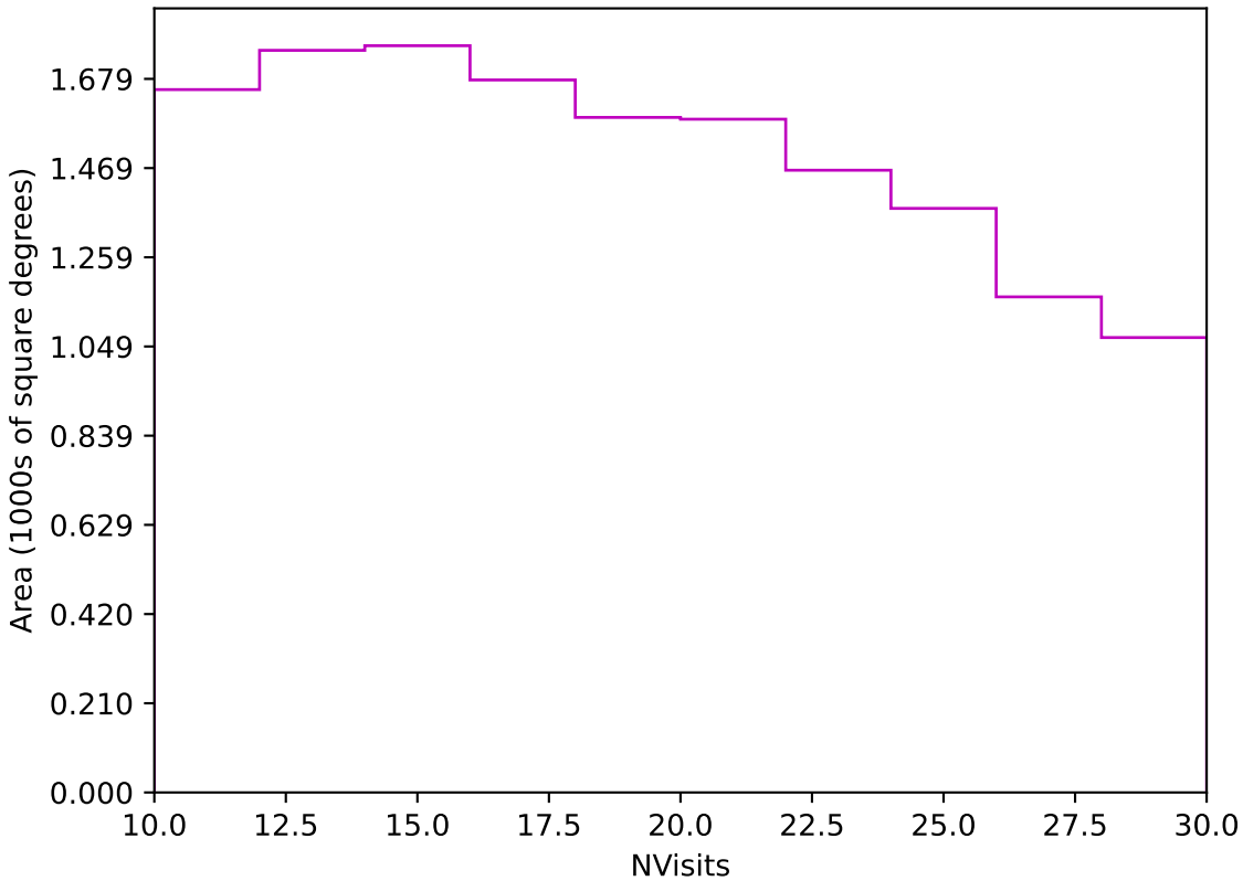
no_high_blob_v3.3_10yrs Yr 3-4 z band: NVisits
