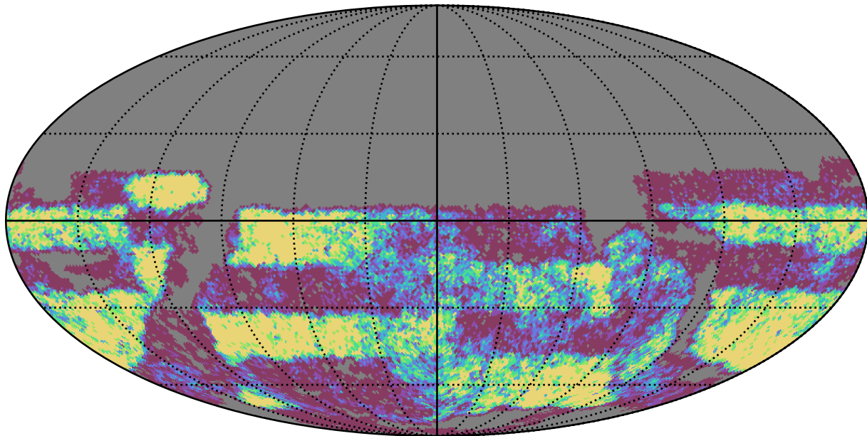
no_high_blob_v3.3_10yrs Yr 3-4 u band: NVisits
