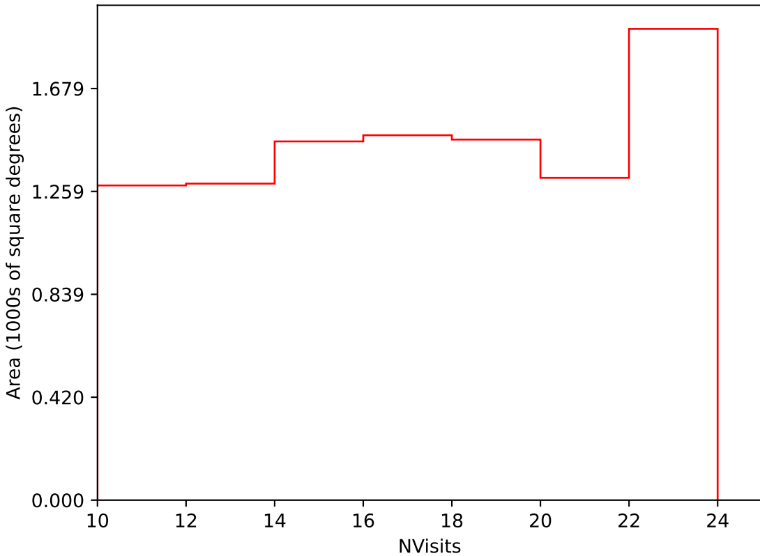
no_high_blob_v3.3_10yrs Yr 3-4 i band: NVisits
