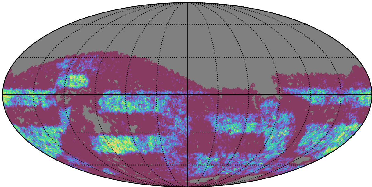
no_high_blob_v3.3_10yrs Yr 3-4 g band: NVisits
