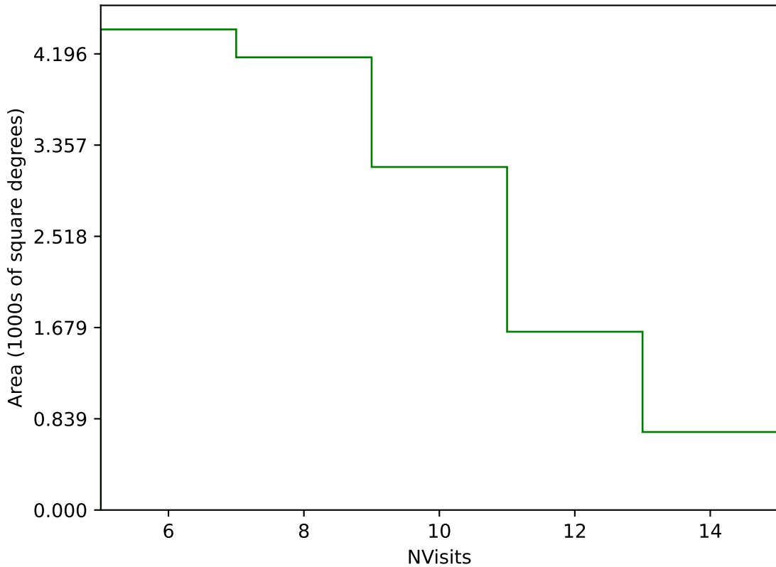
no_high_blob_v3.3_10yrs Yr 3-4 g band: NVisits
